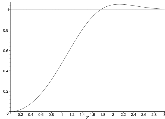
FIGURE 1. The 1-dimensional limit pair correlation function \kappa_{11}
