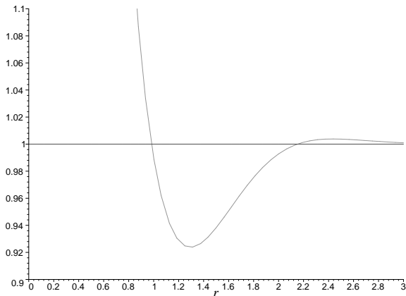
FIGURE 3. The limit pair correlation function \kappa_{12}
