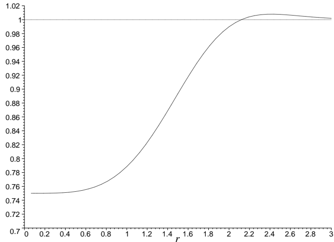
FIGURE 2. The limit pair correlation function \kappa_{22}
